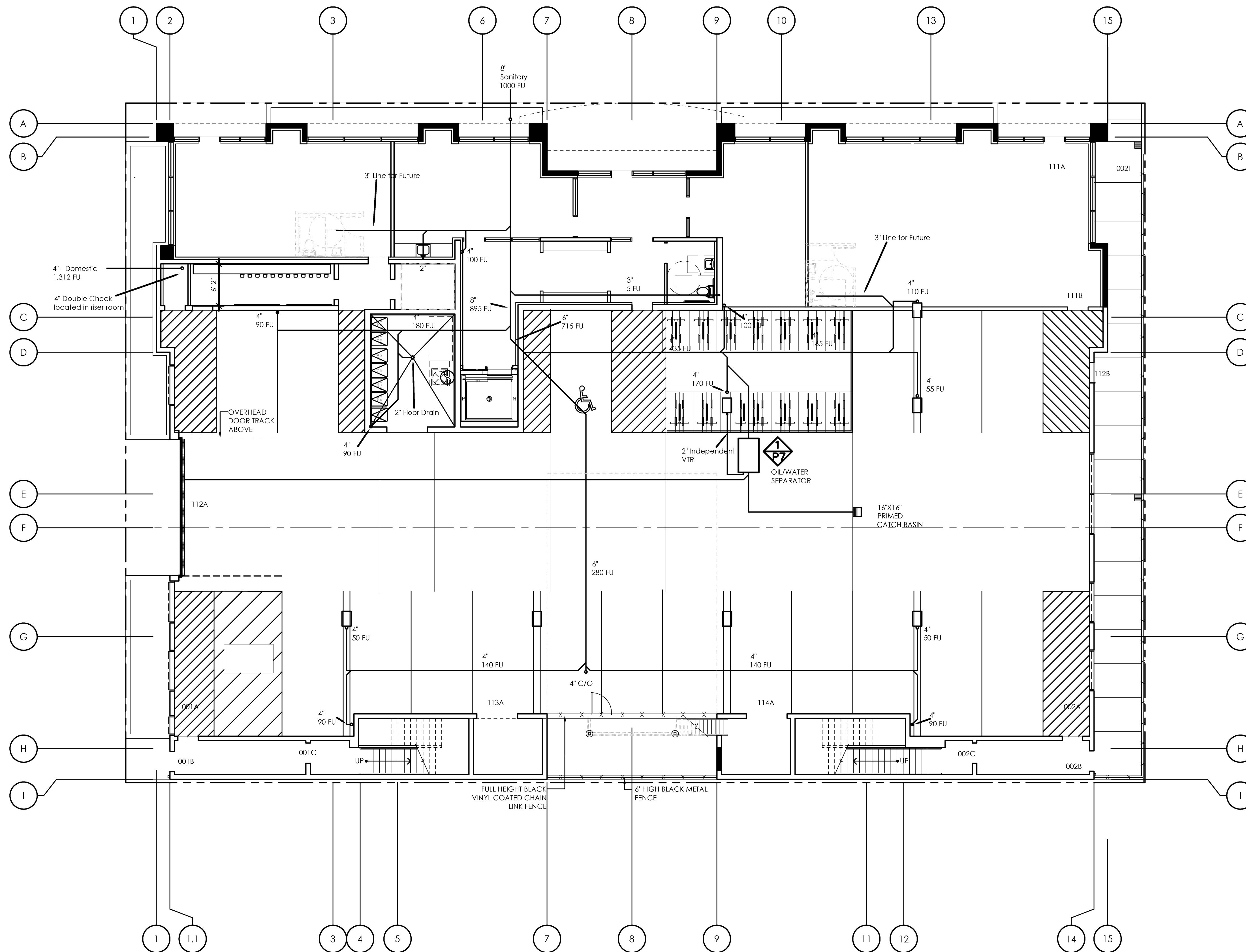
1 FIRST FLOOR UNDERGROUND PLAN P-1
